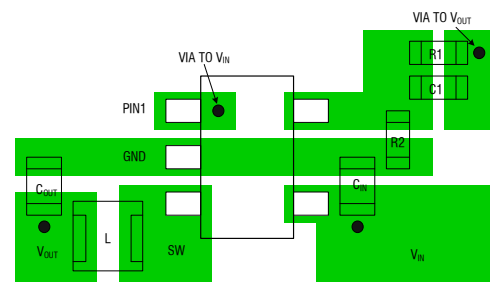
Figure 3. XR3406Suggested Layout
