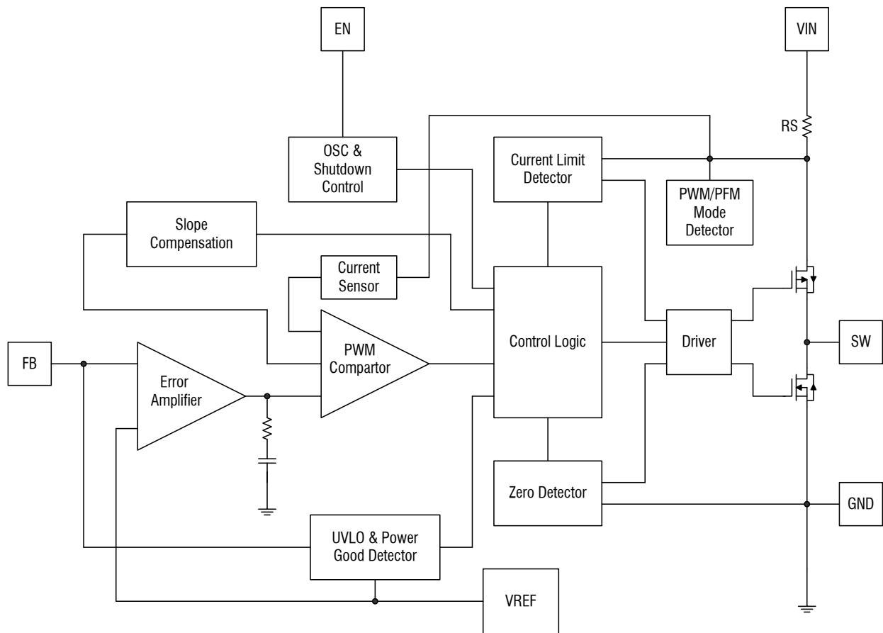
Figure 2. XR3406Block Diagram
