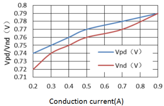
Power transistor diode conduction characteristics
