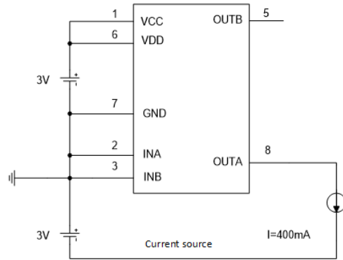
PMOS body diode conduction voltage test schematic
