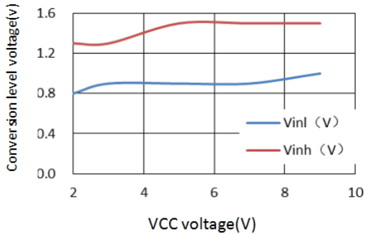
Logic high / low voltage with VCC curve
