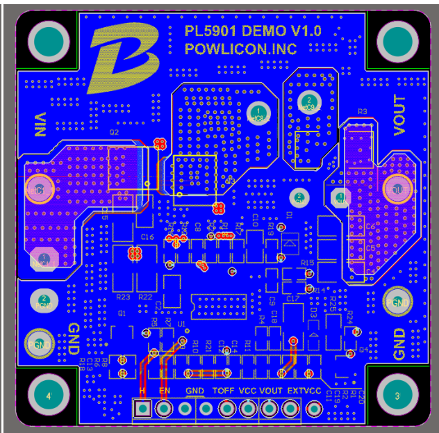
Figure 25. Bottom lay
